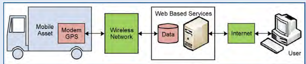
A mobile data platform and data collection system includes an on-board modem and GPS unit and exports data from the vehicle's sensors via a wireless network to a database with a web-based interface.
